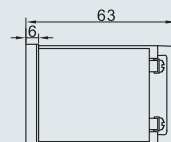
Ammeter (48 type) / Voltmeter (48 type)
