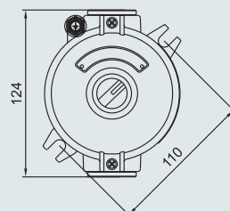
Rotary button
